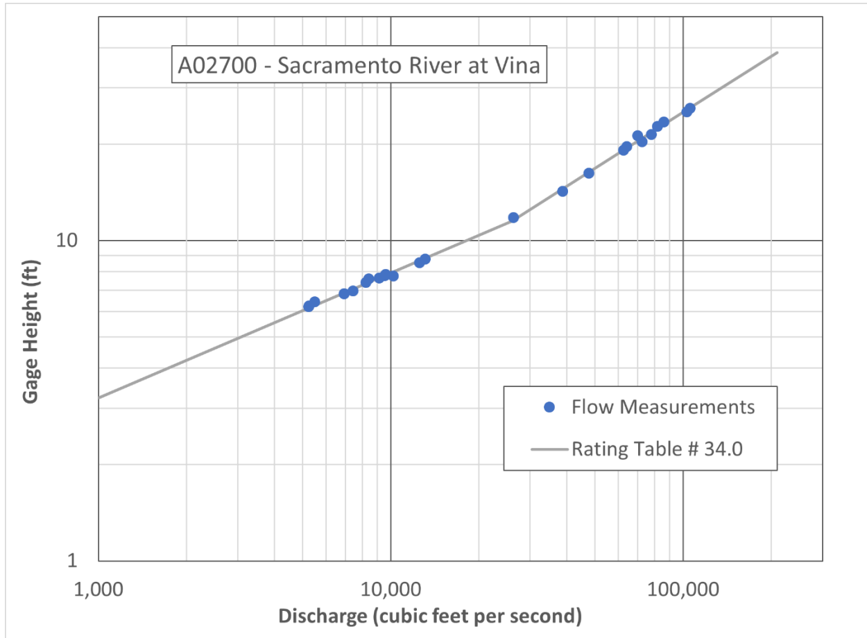
Figure 2 Example stage-discharge rating curve
